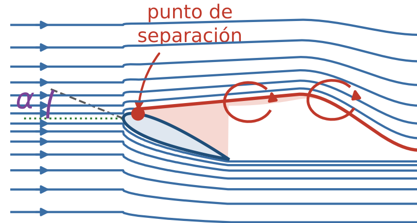
(c) \alpha = 22^\circ > \alpha_{stall}
