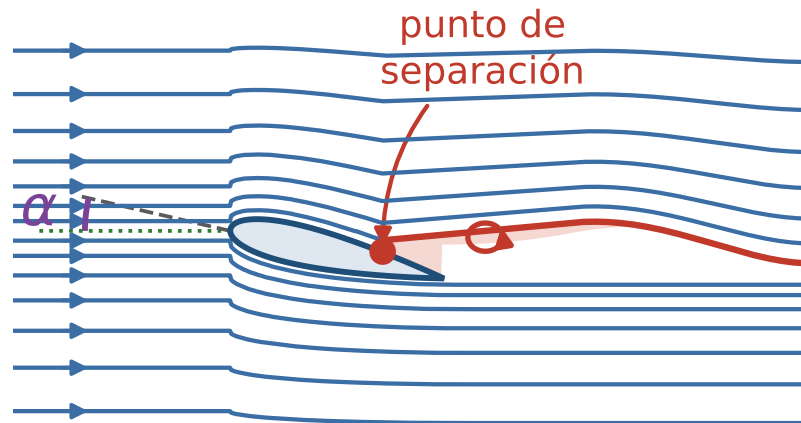
(b) \alpha = 13^\circ \approx \alpha_{stall}
